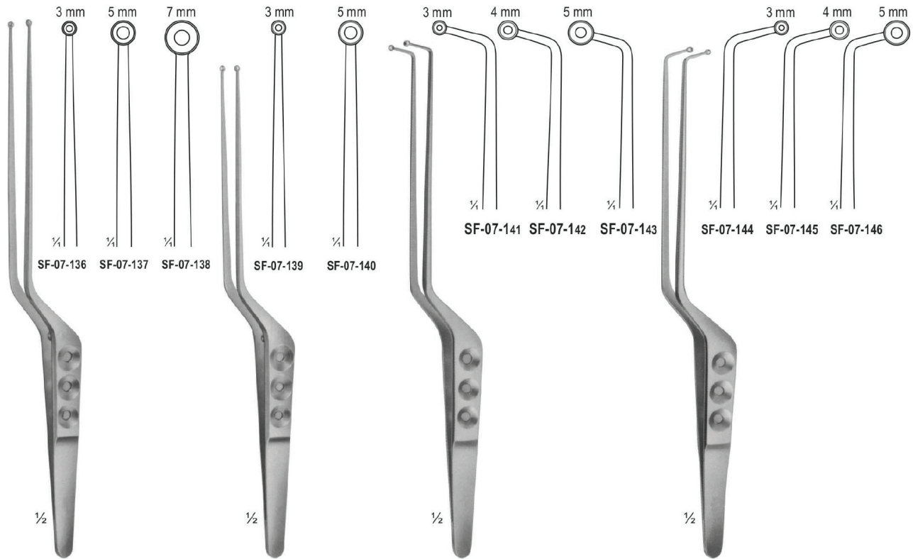
SF-07-136 - SF-07-138 YASARGIL-SAMI Jaws Spoon-Shaped 240 mm
